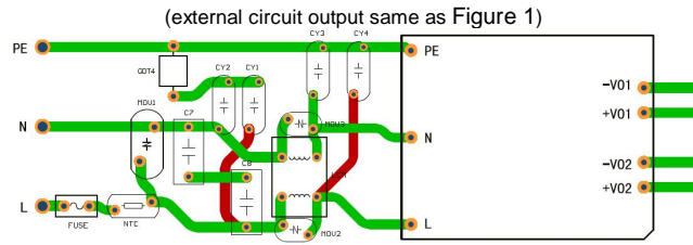
(Figure 4) EMC application circuit PCB layout
